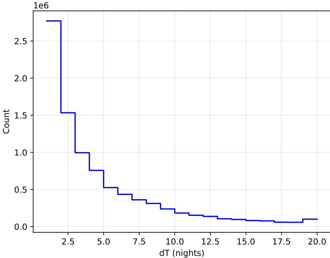
roll_pause_mjdp270_v3.4_10yrs All sky all bands: DeltaNight Histogram
