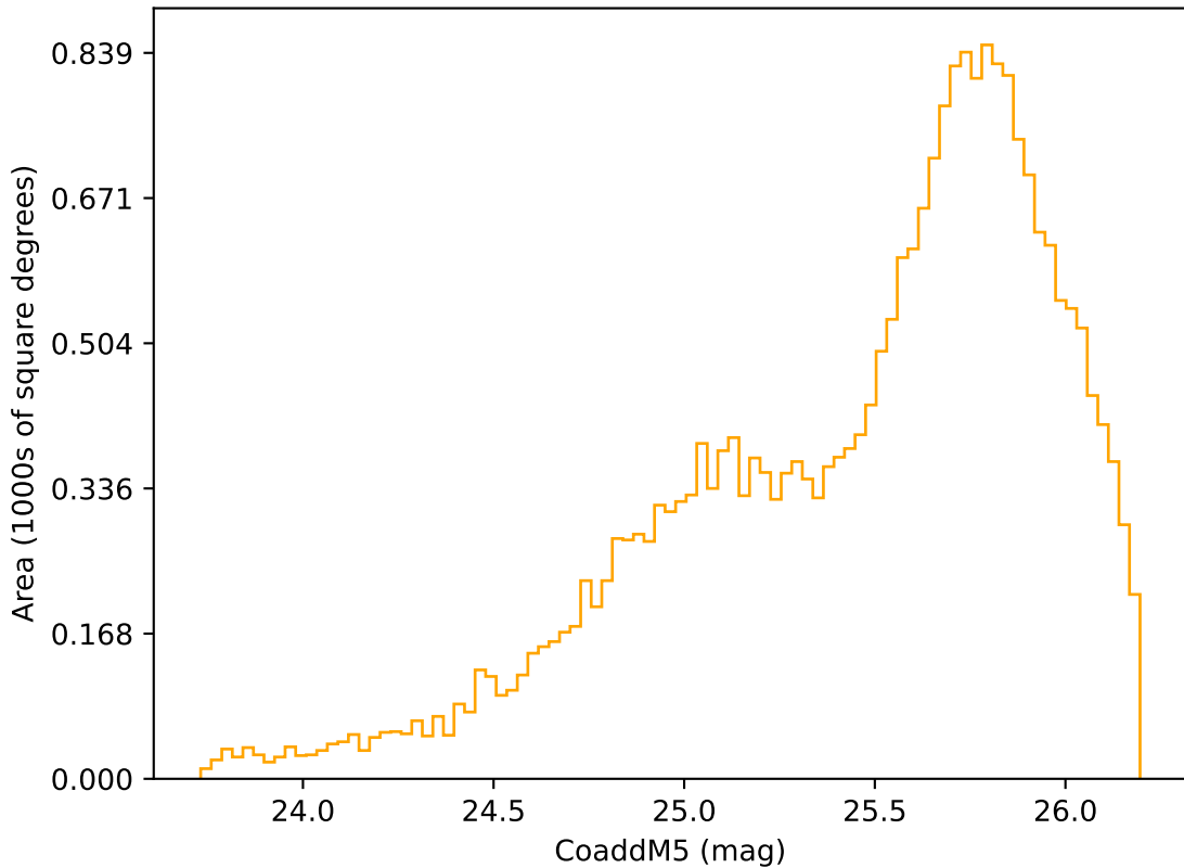
roll_pause_mjdp270_v3.4_10yrs Yr 3-4 r band: CoaddM5
