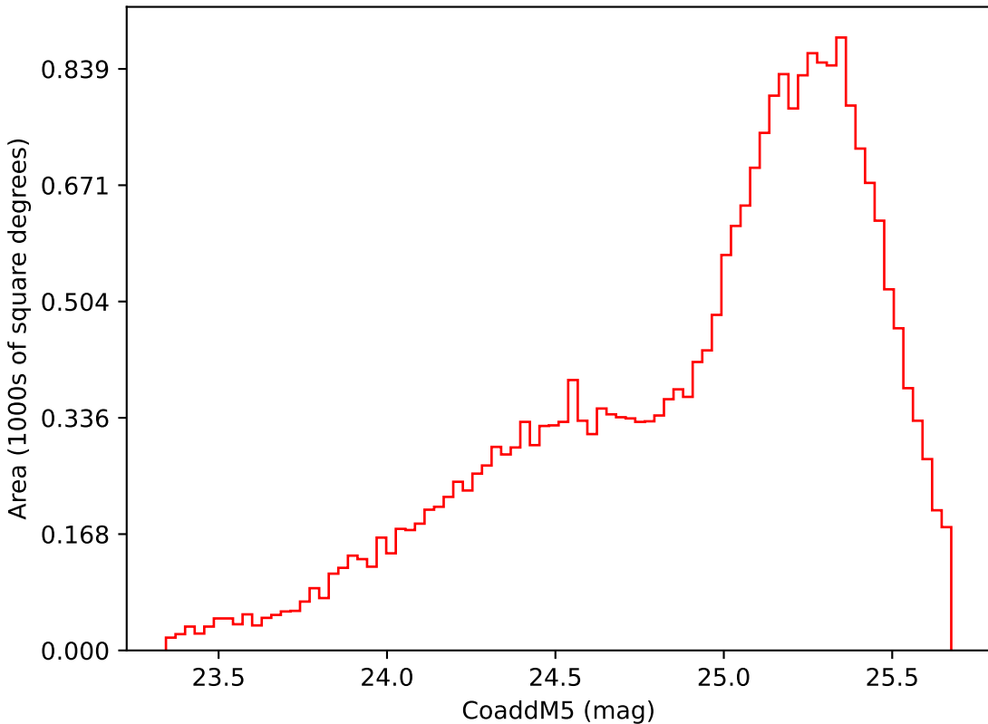
roll_pause_mjdp270_v3.4_10yrs Yr 3-4 i band: CoaddM5
