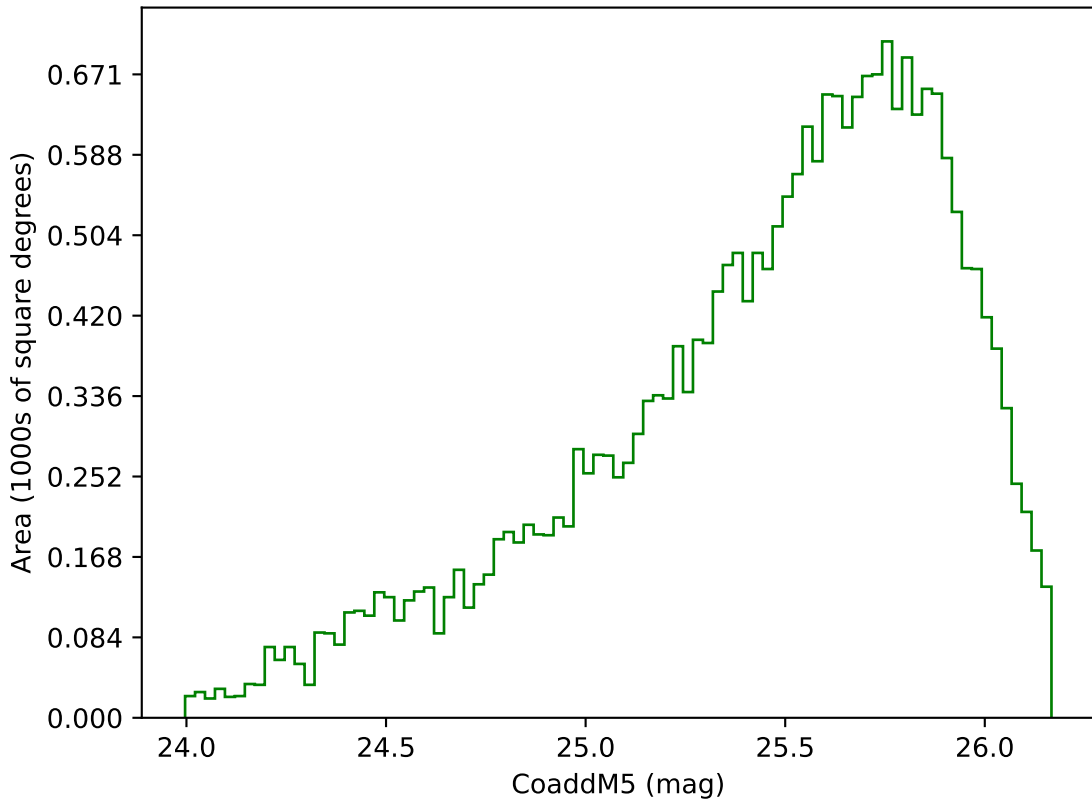
roll_pause_mjdp270_v3.4_10yrs Yr 3-4 g band: CoaddM5
