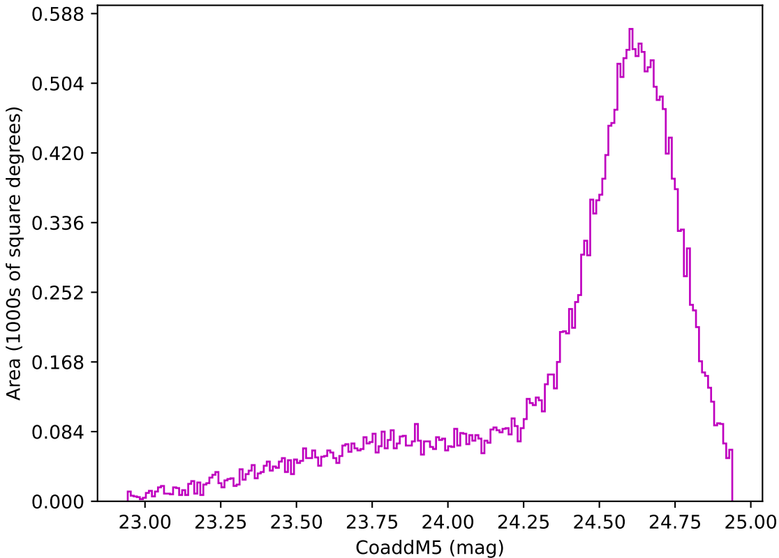
roll_pause_mjdp270_v3.4_10yrs Yr 1 z band: CoaddM5
