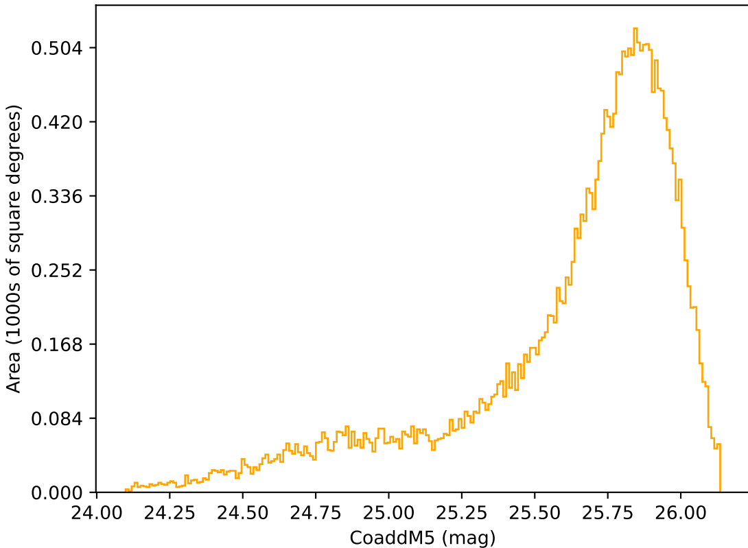
roll_pause_mjdp270_v3.4_10yrs Yr 1 r band: CoaddM5
