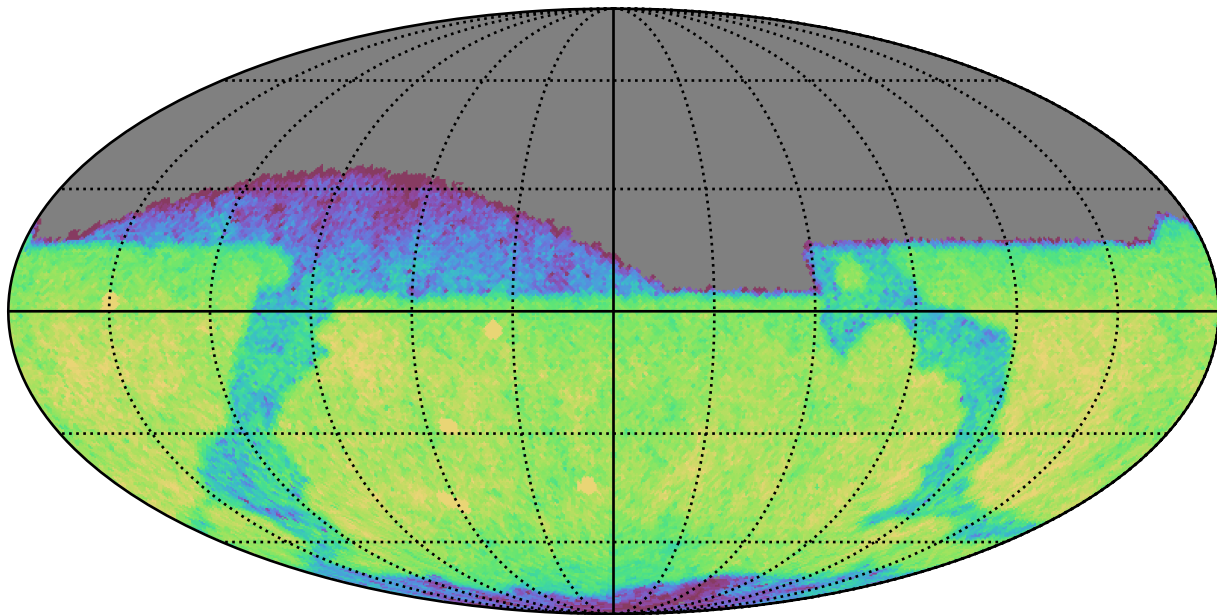
roll_pause_mjdp270_v3.4_10yrs Yr 1 i band: CoaddM5
