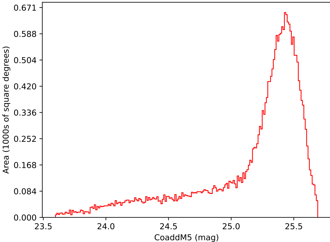
roll_pause_mjdp270_v3.4_10yrs Yr 1 i band: CoaddM5
