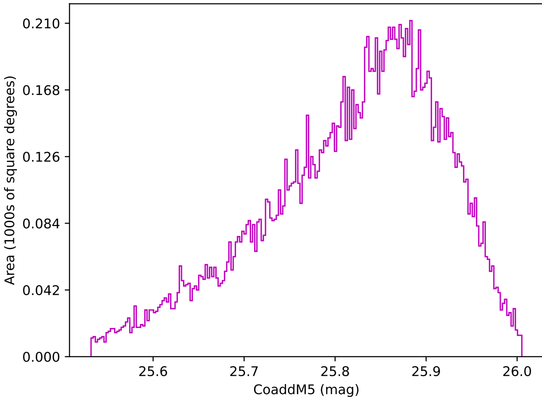
roll_pause_mjdp270_v3.4_10yrs WFD z band: CoaddM5
