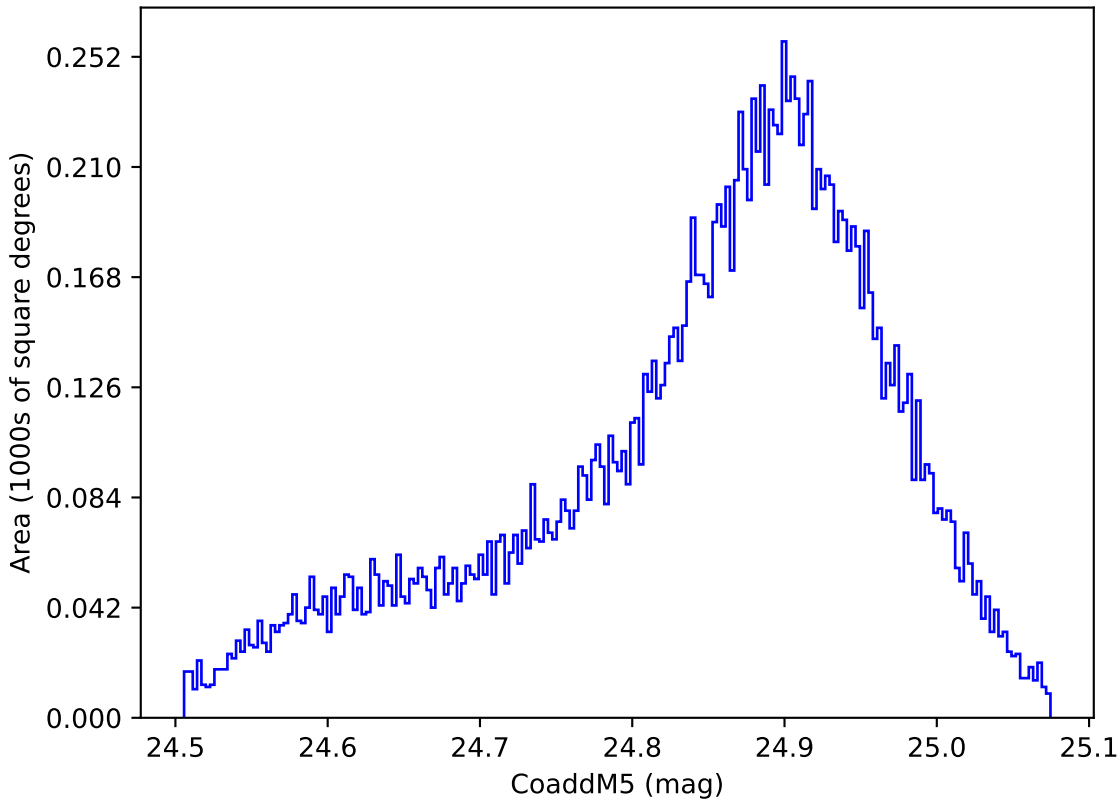
roll_pause_mjdp270_v3.4_10yrs WFD y band: CoaddM5
