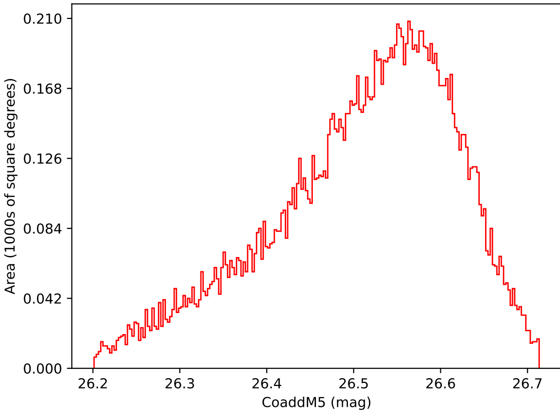
roll_pause_mjdp270_v3.4_10yrs WFD i band: CoaddM5
