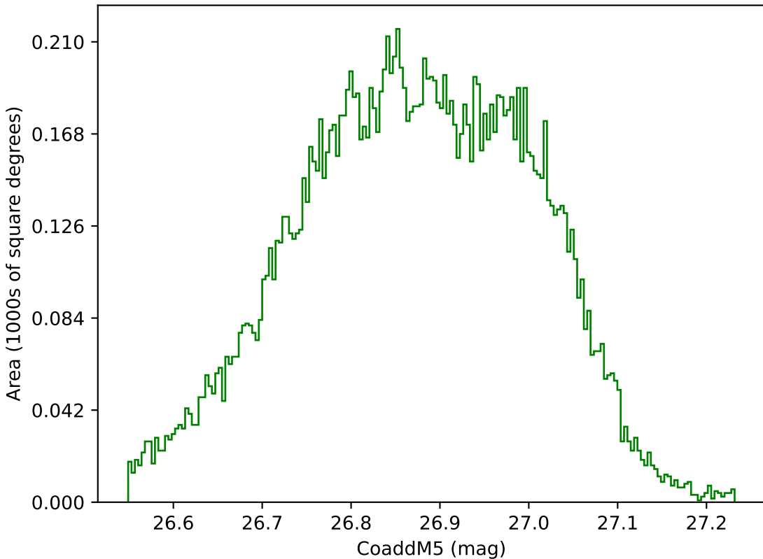
roll_pause_mjdp270_v3.4_10yrs WFD g band: CoaddM5
