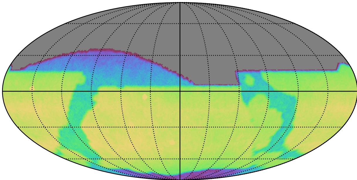
roll_pause_mjdp270_v3.4_10yrs All sky z band: CoaddM5
