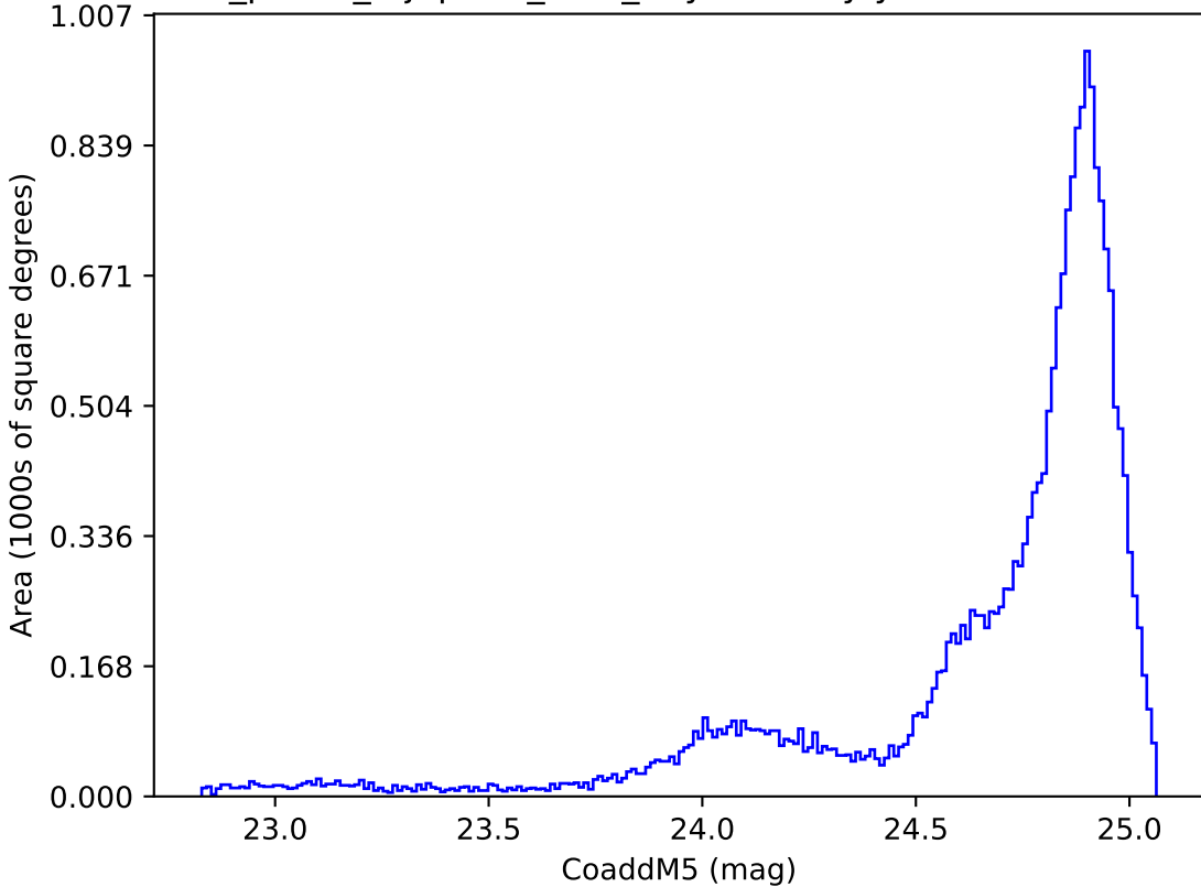
roll_pause_mjdp270_v3.4_10yrs All sky y band: CoaddM5
