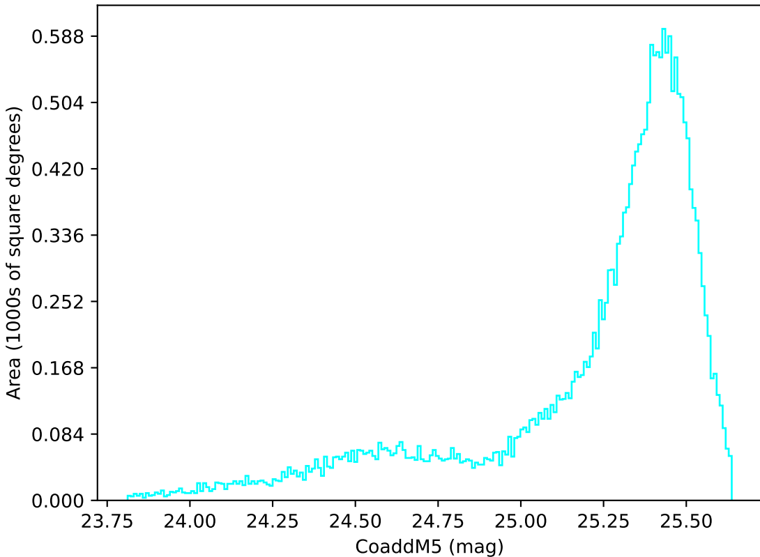
roll_pause_mjdp270_v3.4_10yrs All sky u band: CoaddM5
