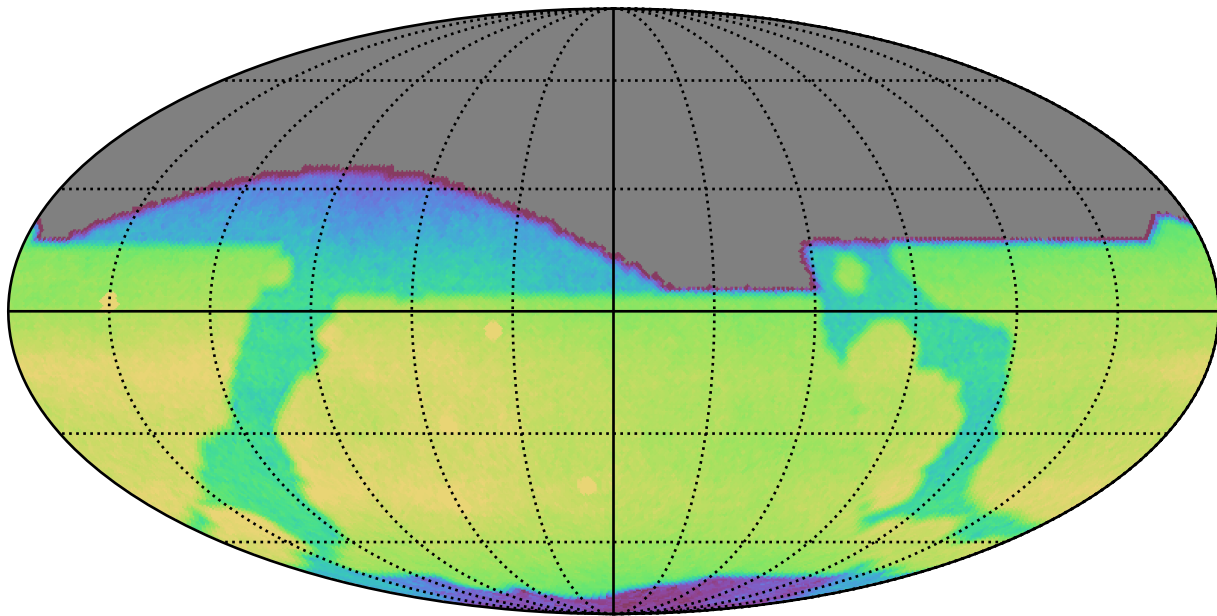
roll_pause_mjdp270_v3.4_10yrs All sky r band: CoaddM5
