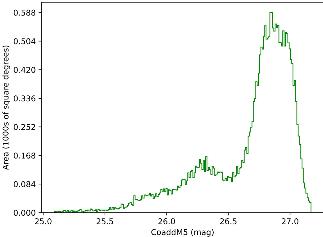
roll_pause_mjdp270_v3.4_10yrs All sky g band: CoaddM5
