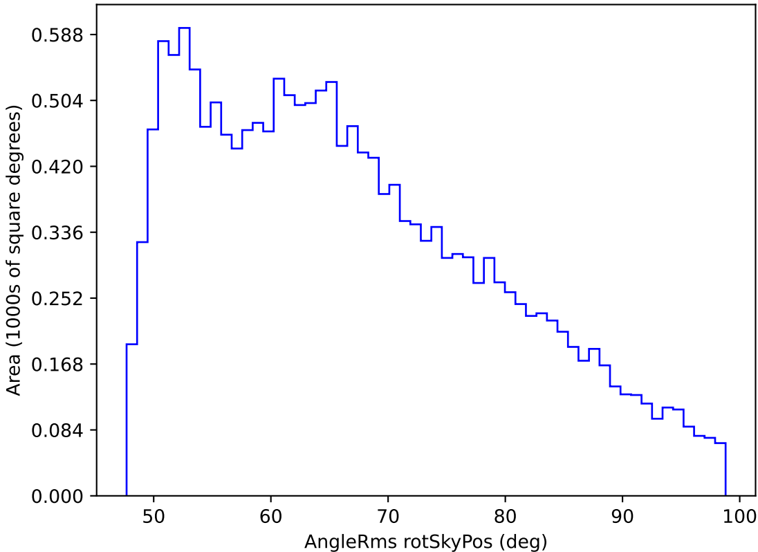
roll_pause_mjdp270_v3.4_10yrs WFD r band: AngleRms rotSkyPos
