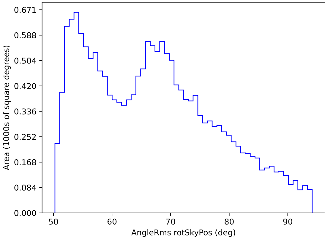
roll_pause_mjdp270_v3.4_10yrs WFD all bands: AngleRms rotSkyPos
