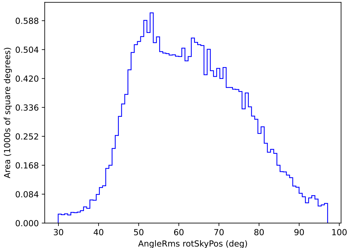
roll_pause_mjdp270_v3.4_10yrs All sky u band: AngleRms rotSkyPos
