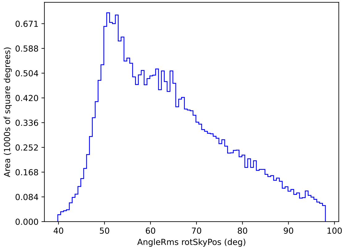
roll_pause_mjdp270_v3.4_10yrs All sky r band: AngleRms rotSkyPos
