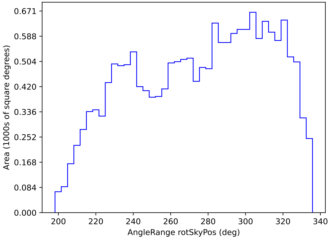
roll_pause_mjdp270_v3.4_10yrs WFD y band: AngleRange rotSkyPos
