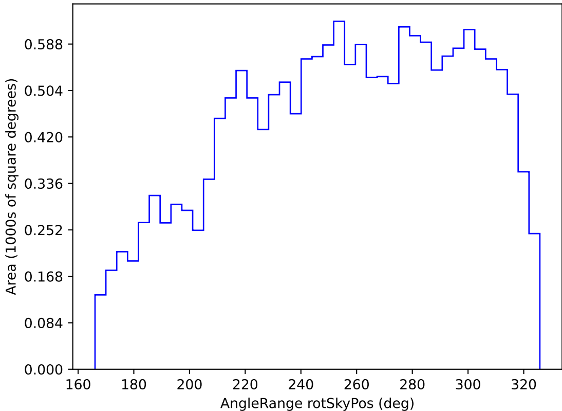
roll_pause_mjdp270_v3.4_10yrs WFD u band: AngleRange rotSkyPos
