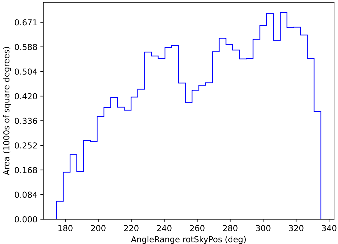
roll_pause_mjdp270_v3.4_10yrs WFD g band: AngleRange rotSkyPos
