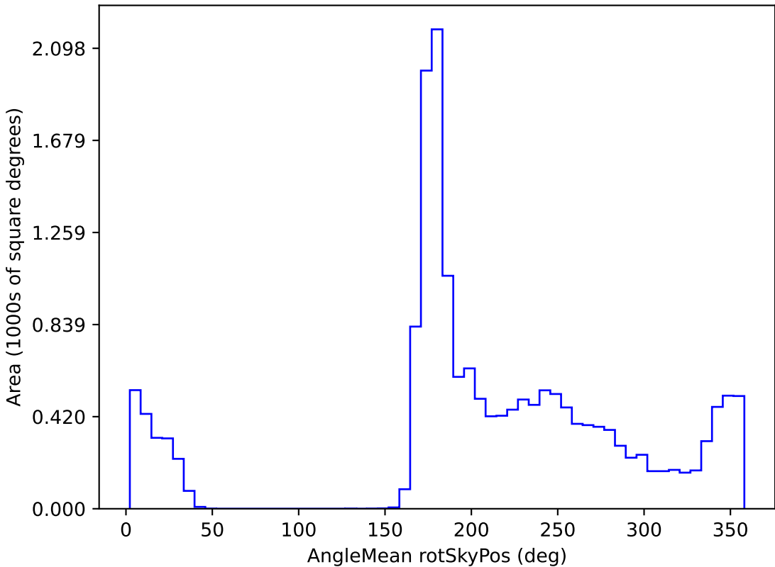
roll_pause_mjdp270_v3.4_10yrs WFD z band: AngleMean rotSkyPos
