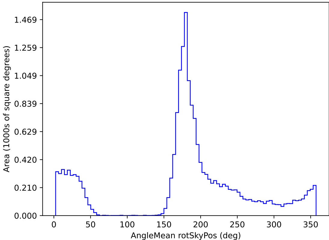
roll_pause_mjdp270_v3.4_10yrs WFD g band: AngleMean rotSkyPos
