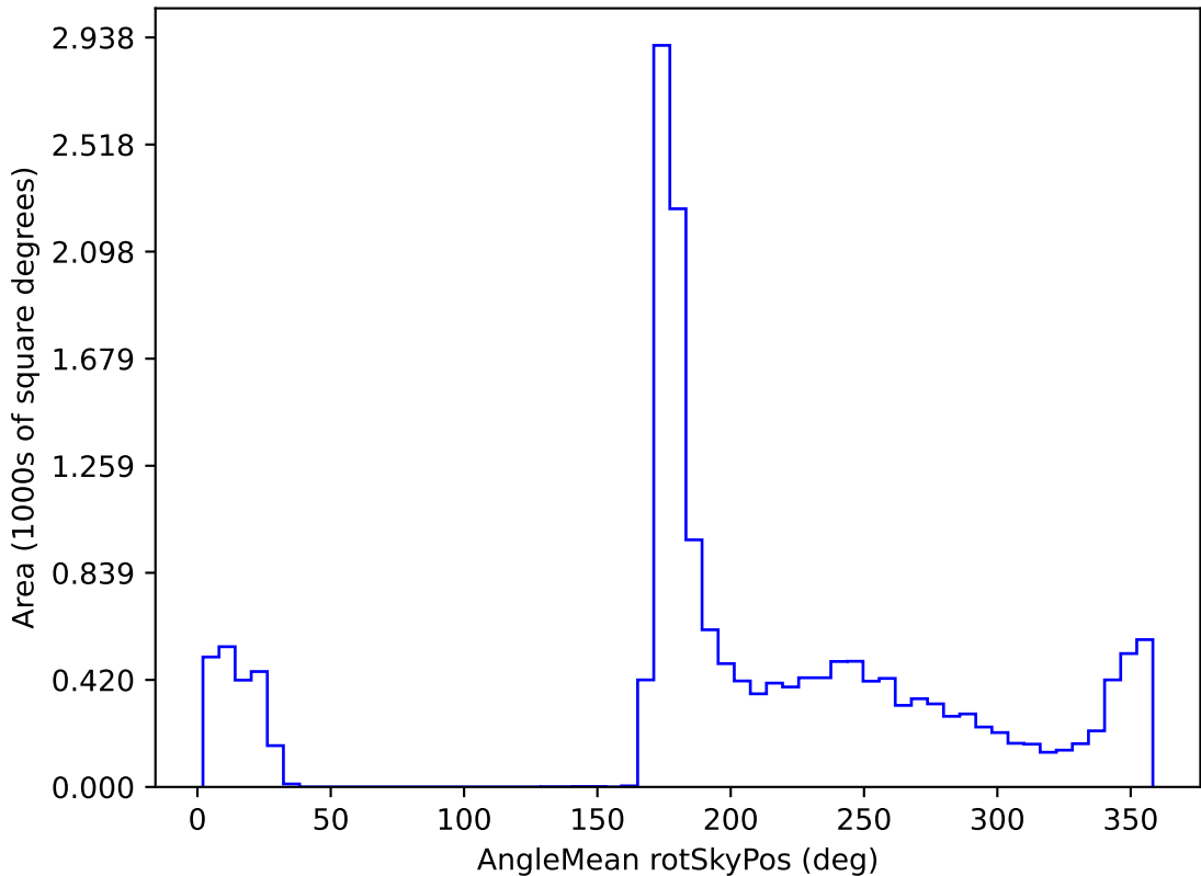
roll_pause_mjdp270_v3.4_10yrs WFD all bands: AngleMean rotSkyPos
