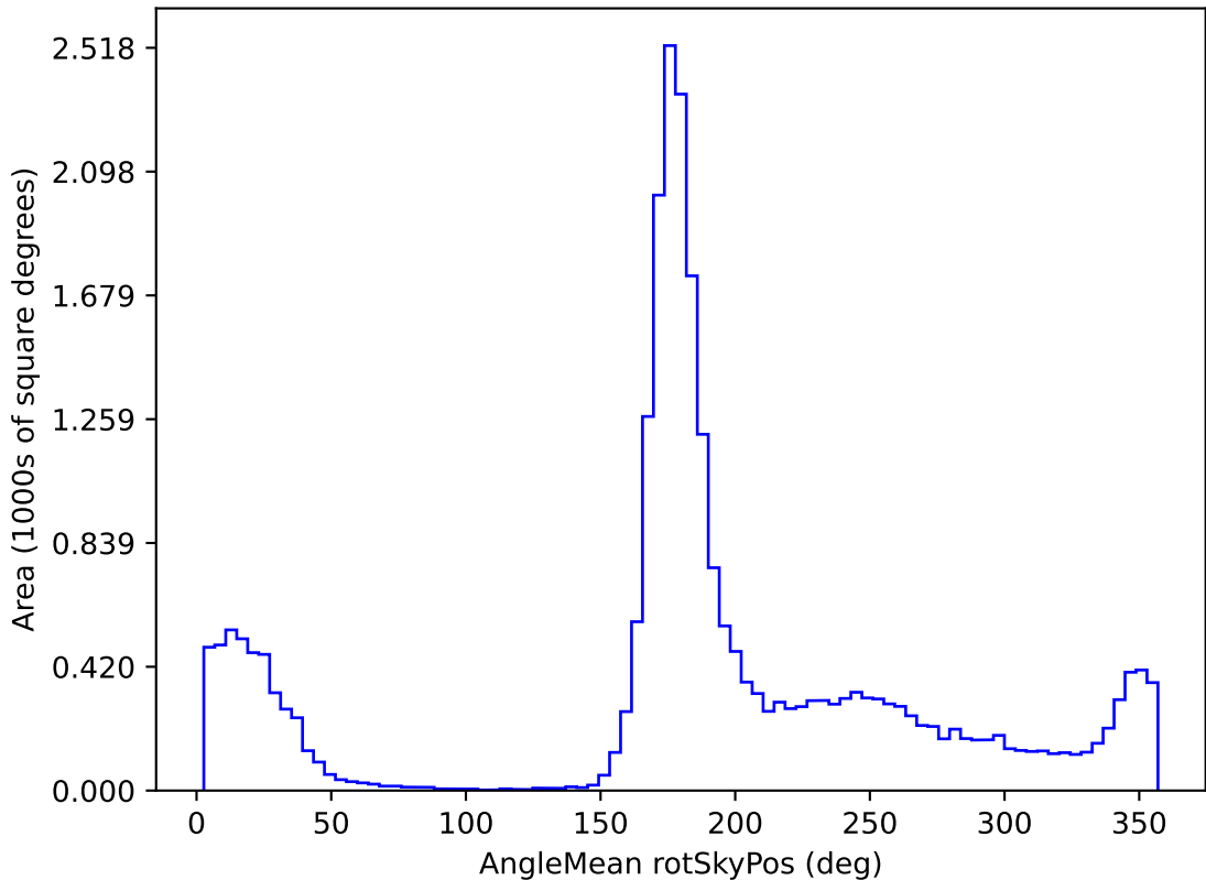
roll_pause_mjdp270_v3.4_10yrs All sky r band: AngleMean rotSkyPos
