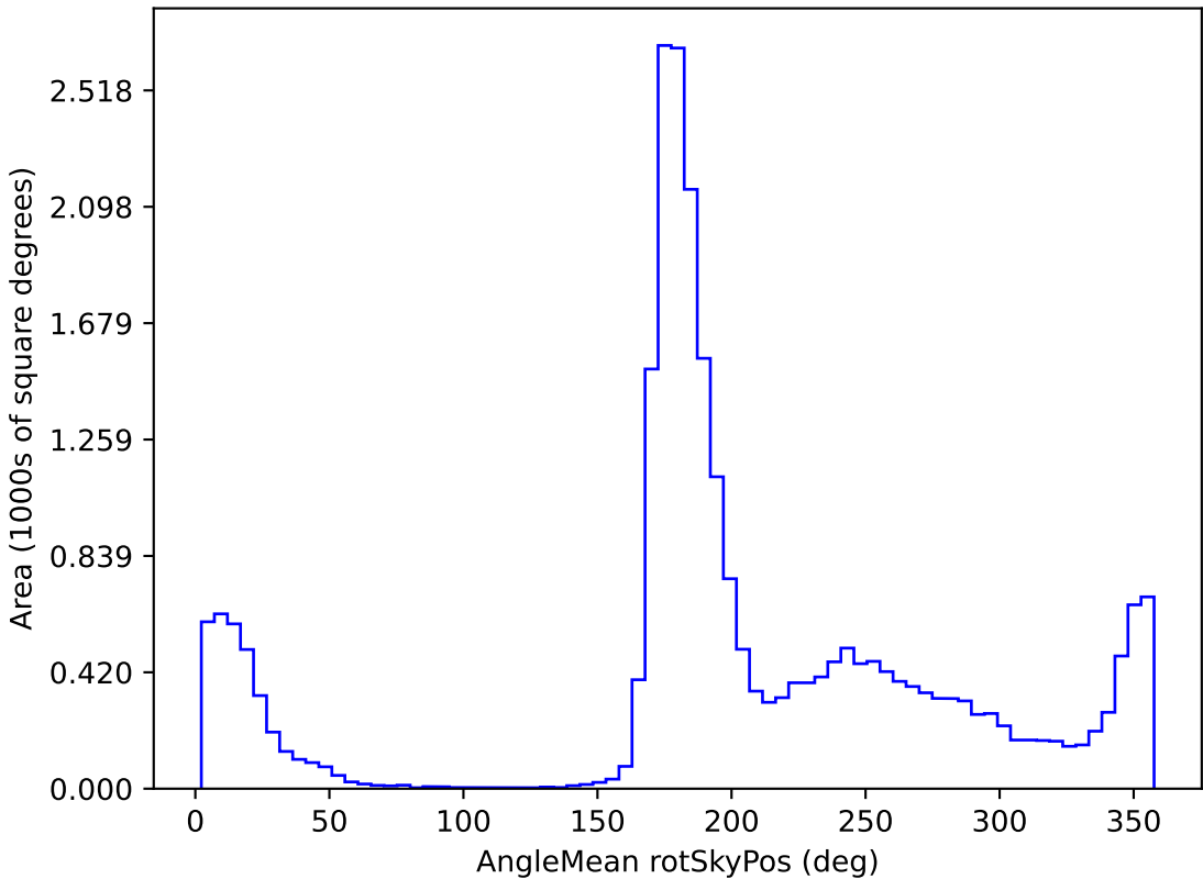
roll_pause_mjdp270_v3.4_10yrs All sky i band: AngleMean rotSkyPos
