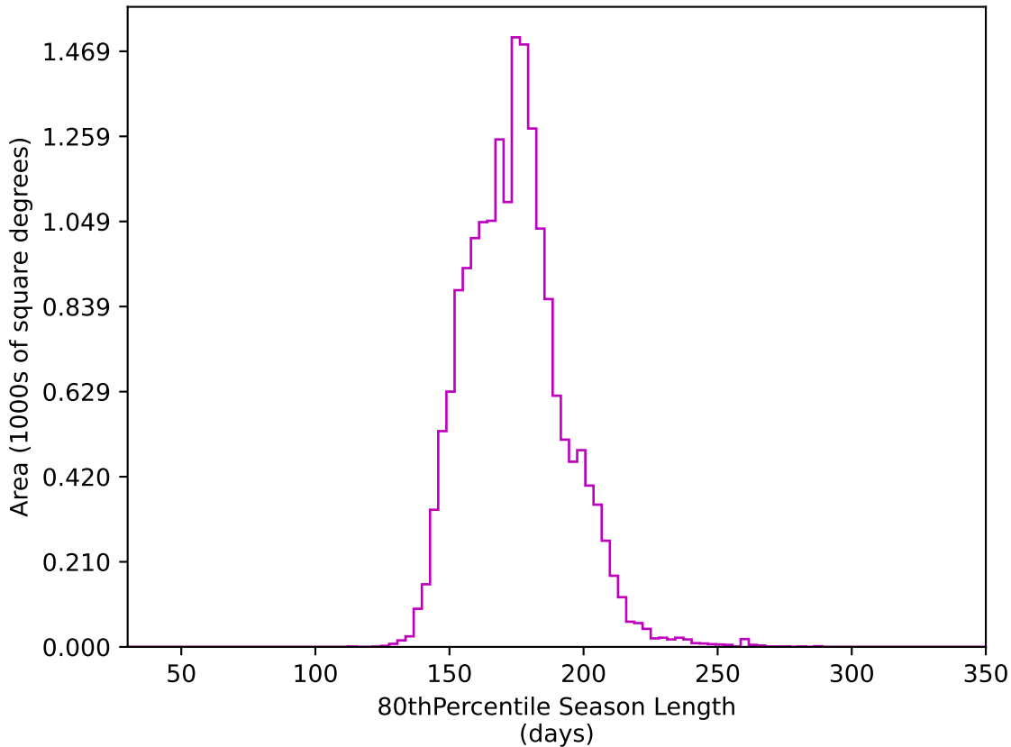
roll_pause_mjdp270_v3.4_10yrs WFD z band: 80thPercentile Season Length
