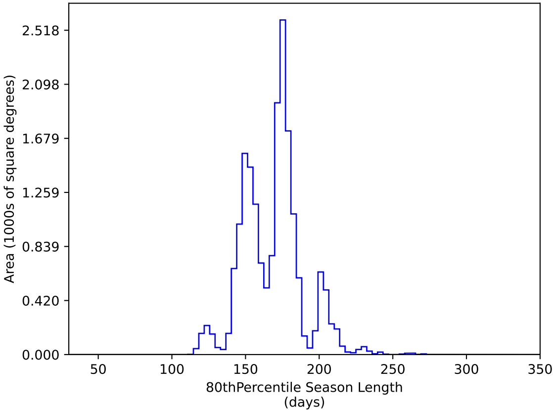
roll_pause_mjdp270_v3.4_10yrs WFD y band: 80thPercentile Season Length
