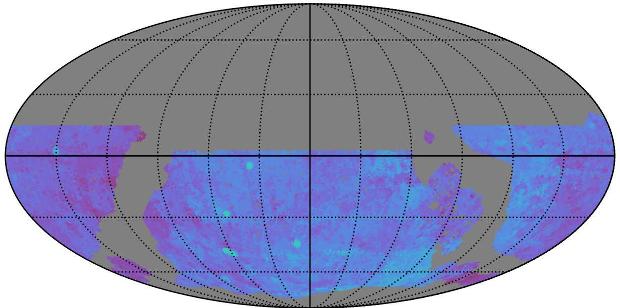
roll_pause_mjdp270_v3.4_10yrs WFD u band: 80thPercentile Season Length
