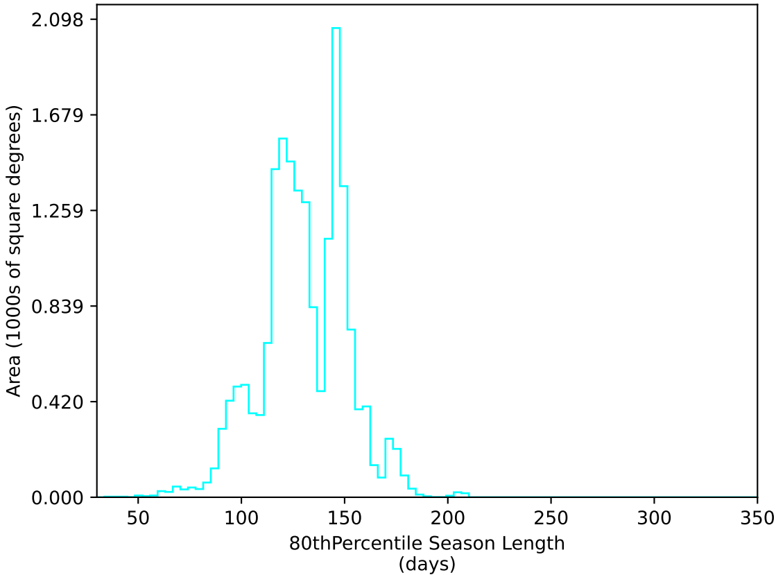
roll_pause_mjdp270_v3.4_10yrs WFD u band: 80thPercentile Season Length
