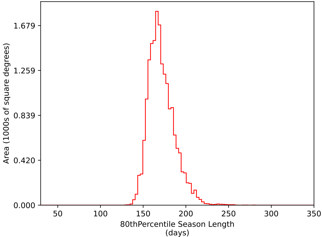
roll_pause_mjdp270_v3.4_10yrs WFD i band: 80thPercentile Season Length
