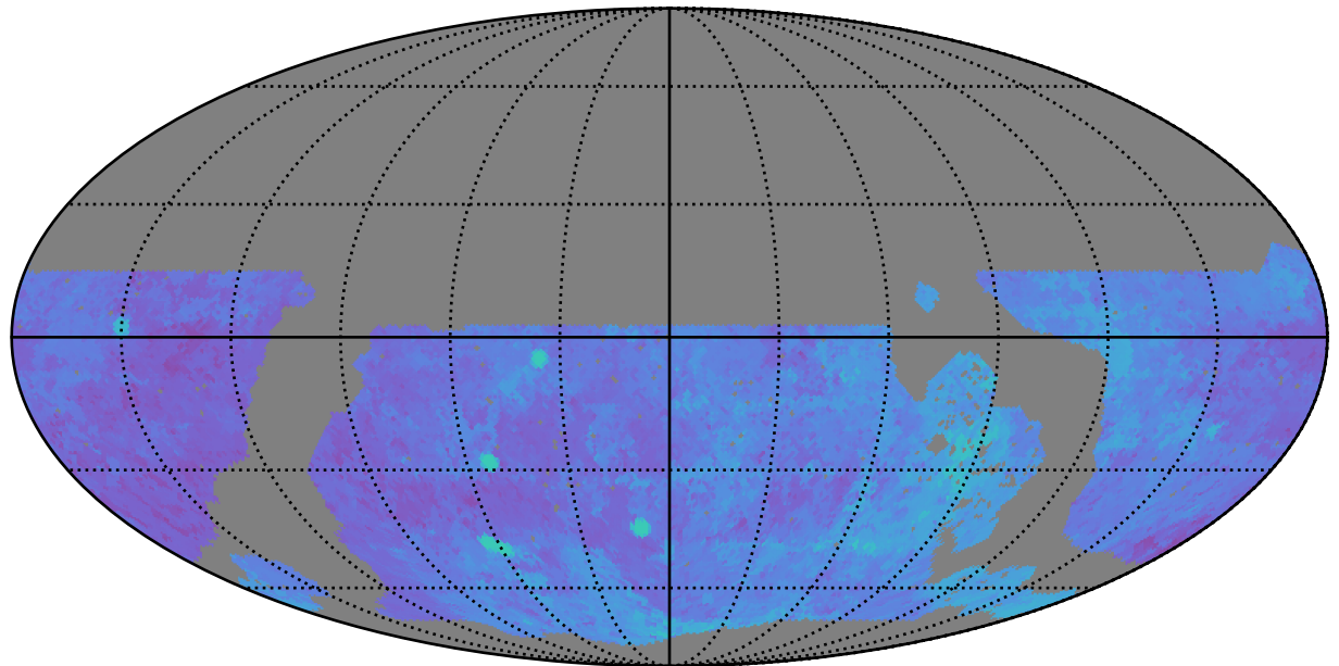
roll_pause_mjdp270_v3.4_10yrs WFD g band: 80thPercentile Season Length
