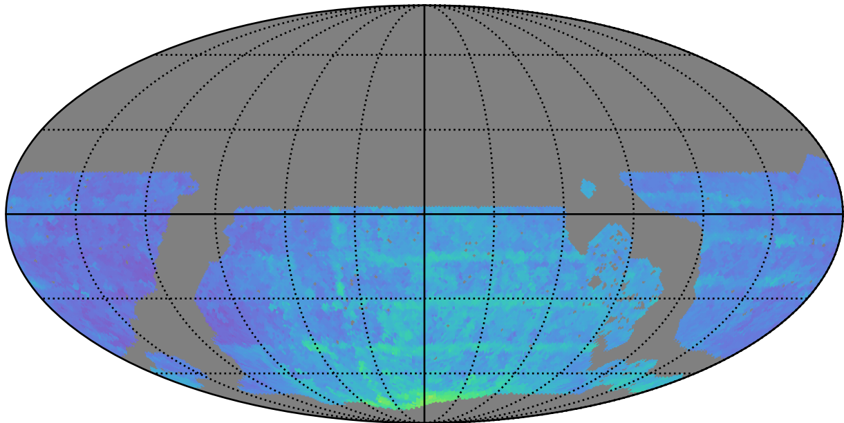
roll_pause_mjdp270_v3.4_10yrs WFD all bands: 80thPercentile Season Length
