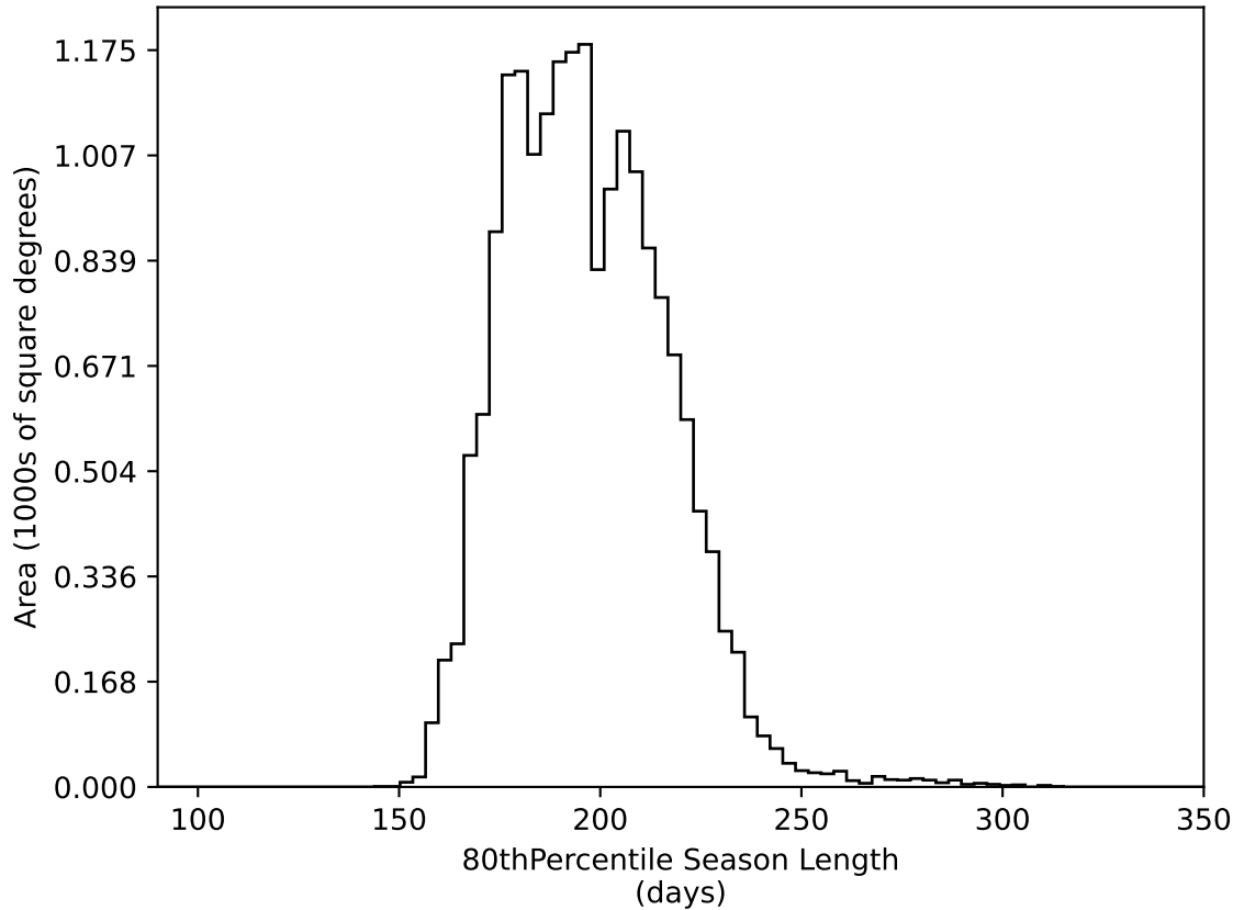
roll_pause_mjdp270_v3.4_10yrs WFD all bands: 80thPercentile Season Length
