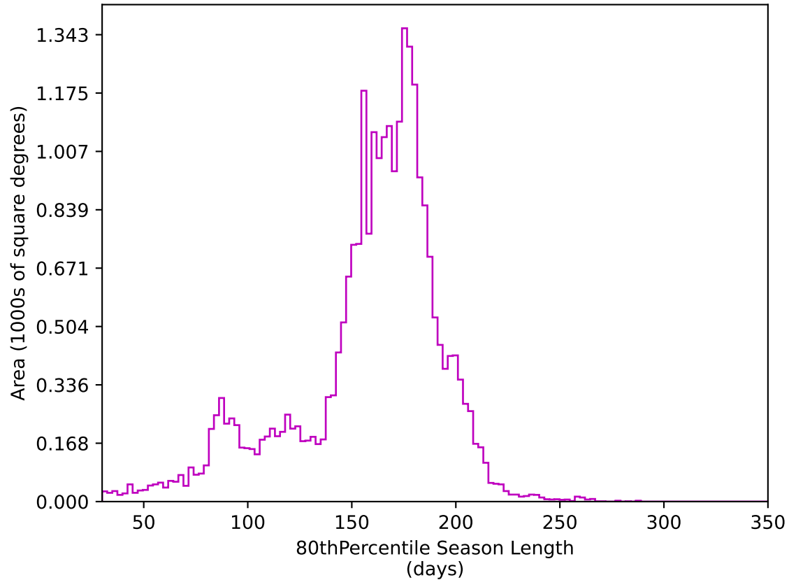
roll_pause_mjdp270_v3.4_10yrs All sky z band: 80thPercentile Season Length
