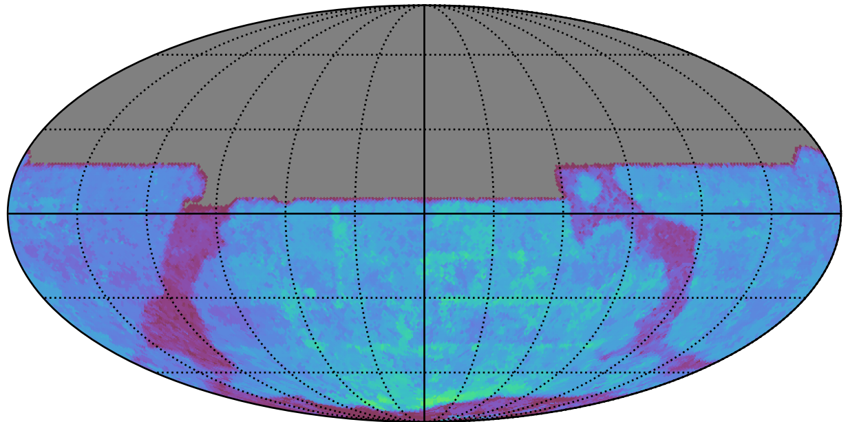
roll_pause_mjdp270_v3.4_10yrs All sky y band: 80thPercentile Season Length
