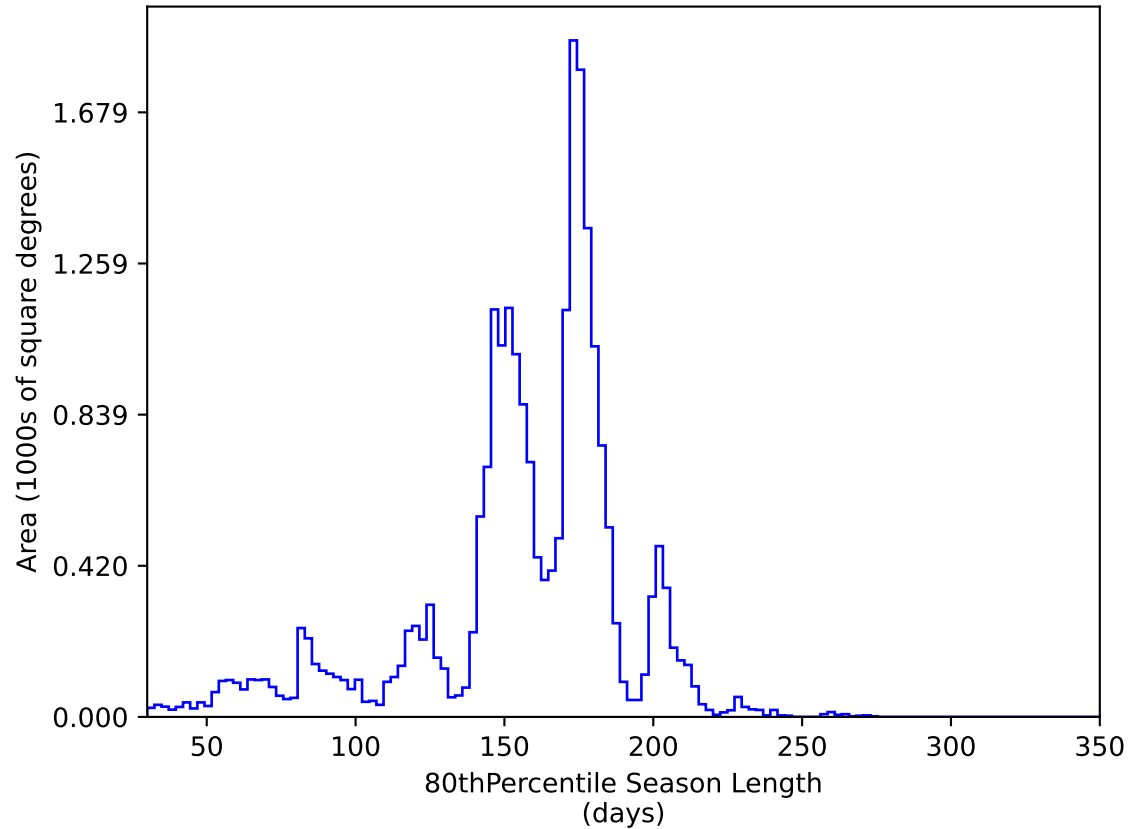
roll_pause_mjdp270_v3.4_10yrs All sky y band: 80thPercentile Season Length
