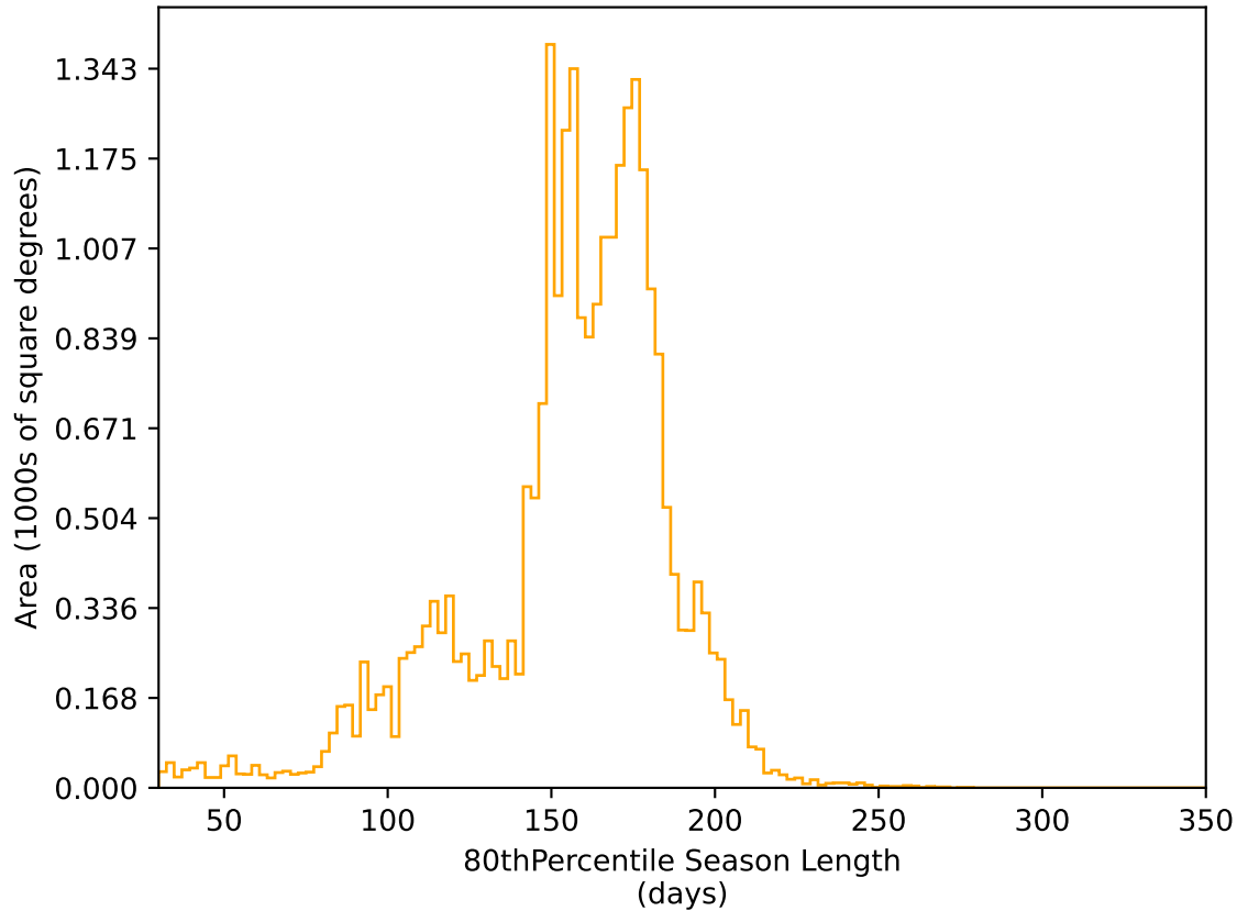
roll_pause_mjdp270_v3.4_10yrs All sky r band: 80thPercentile Season Length
