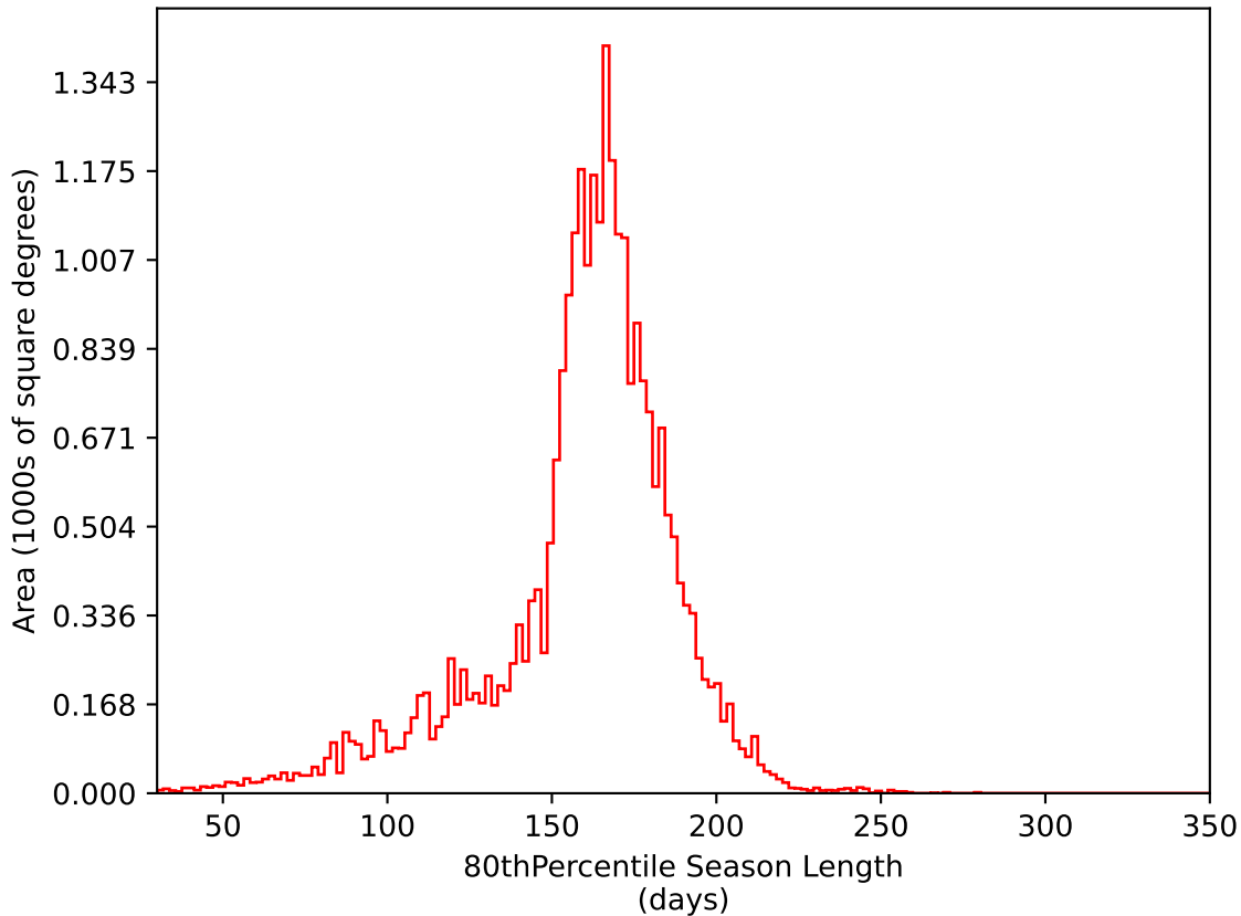
roll_pause_mjdp270_v3.4_10yrs All sky i band: 80thPercentile Season Length
