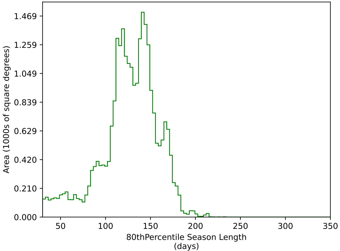
roll_pause_mjdp270_v3.4_10yrs All sky g band: 80thPercentile Season Length
