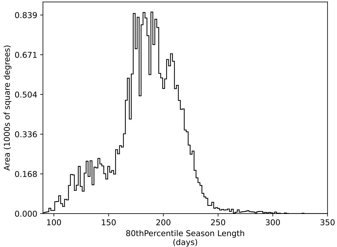
roll_pause_mjdp270_v3.4_10yrs All sky all bands: 80thPercentile Season Length
