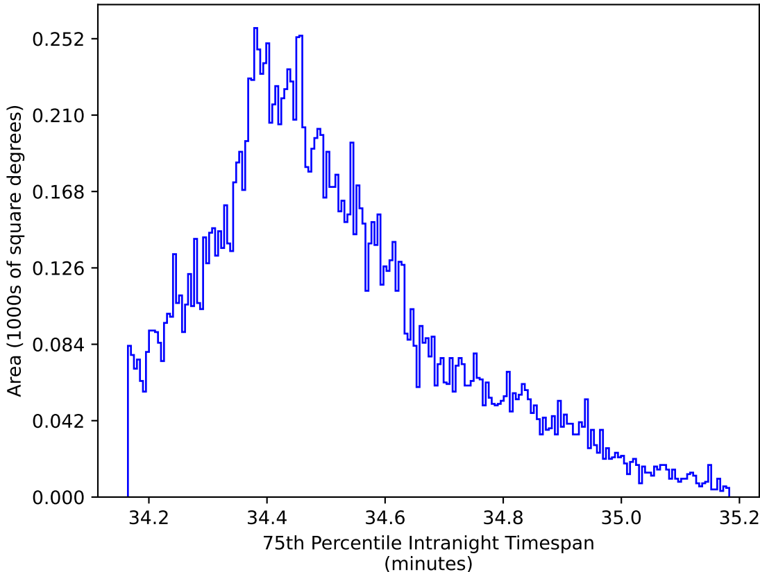
roll_pause_mjdp270_v3.4_10yrs WFD zy bands: 75th Percentile Intranight Timespan
