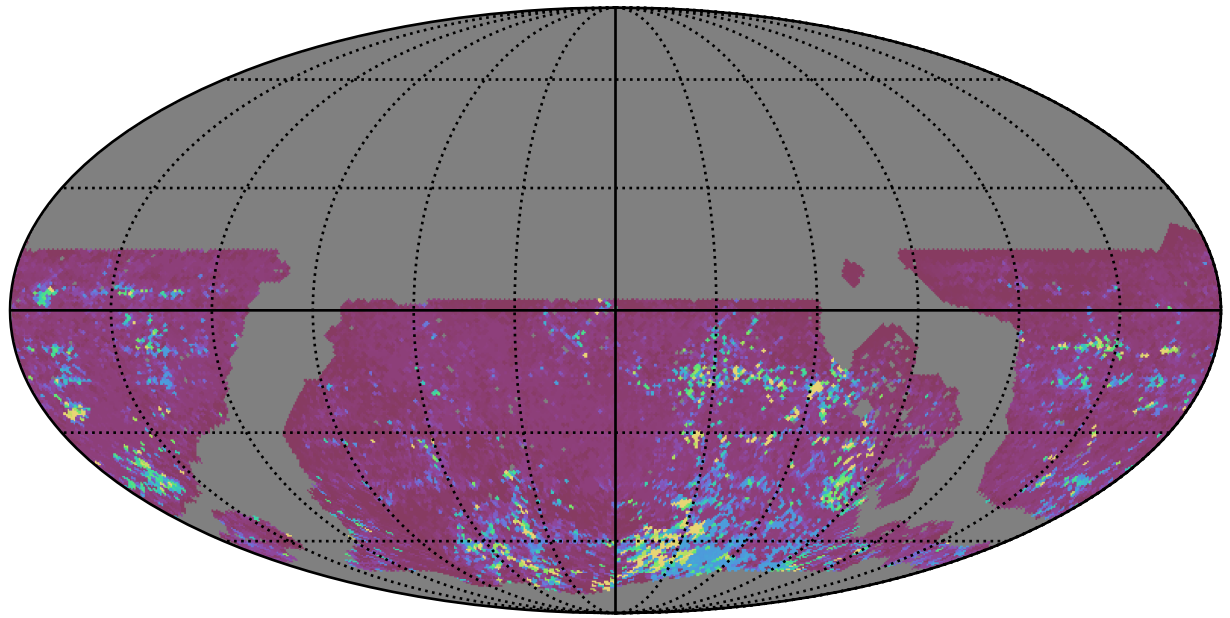
roll_pause_mjdp270_v3.4_10yrs WFD z band: 75th Percentile Intranight Timespan
