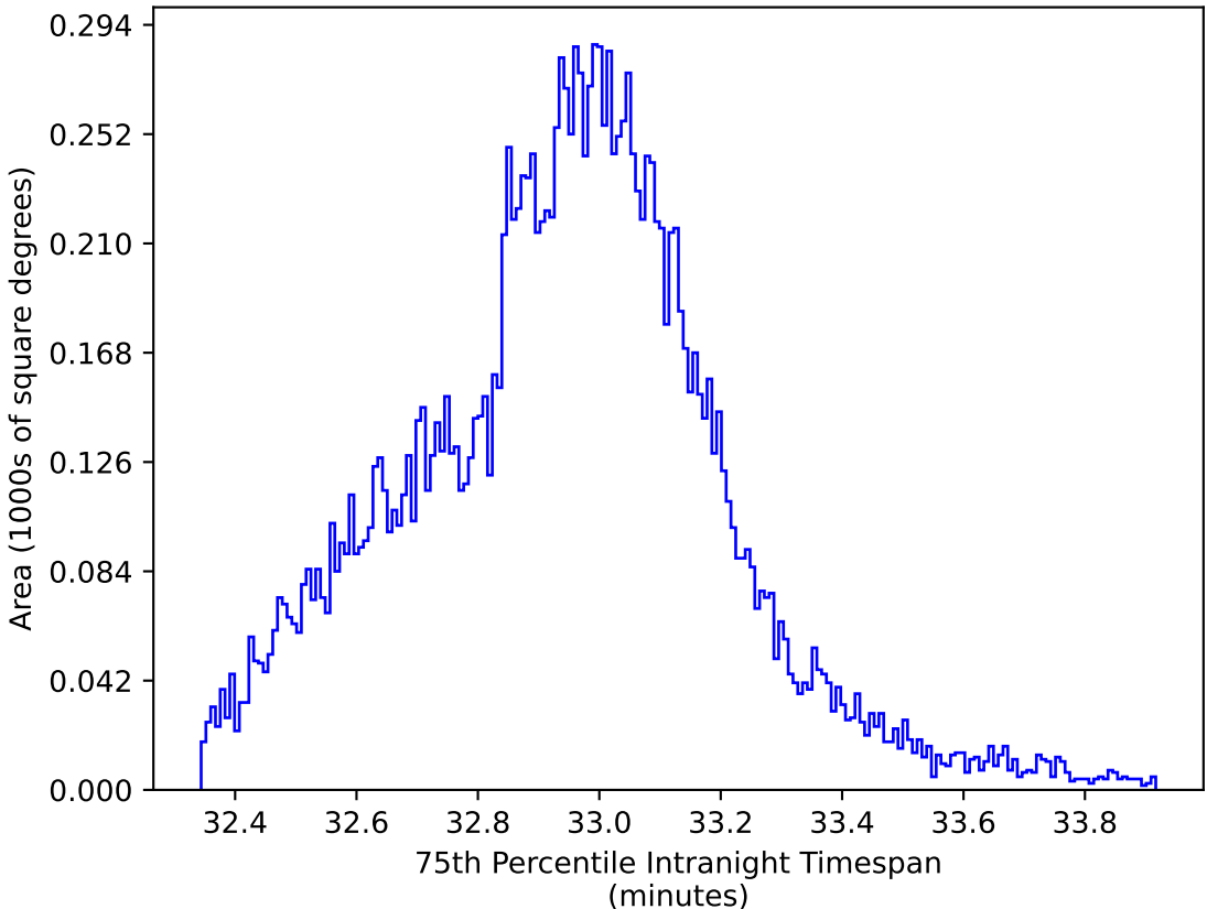
roll_pause_mjdp270_v3.4_10yrs WFD y band: 75th Percentile Intranight Timespan
