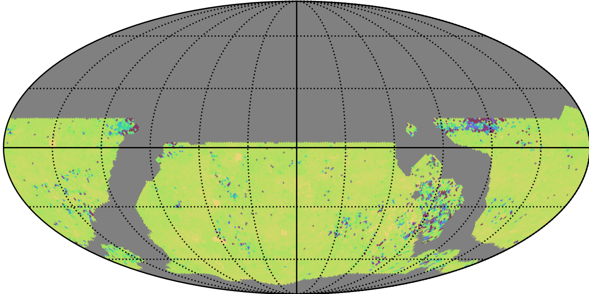
roll_pause_mjdp270_v3.4_10yrs WFD ug bands: 75th Percentile Intranight Timespan
