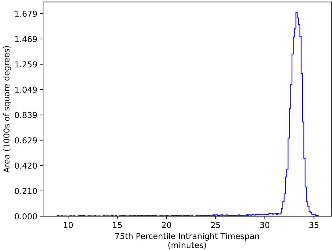
roll_pause_mjdp270_v3.4_10yrs WFD ug bands: 75th Percentile Intranight Timespan
