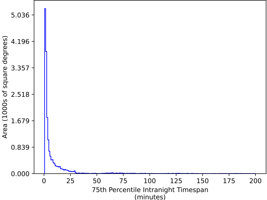
roll_pause_mjdp270_v3.4_10yrs WFD u band: 75th Percentile Intranight Timespan
